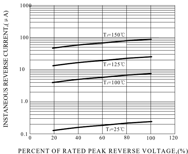
FIG.5-TYPICAL REVERSE CHARACTERISTICS
