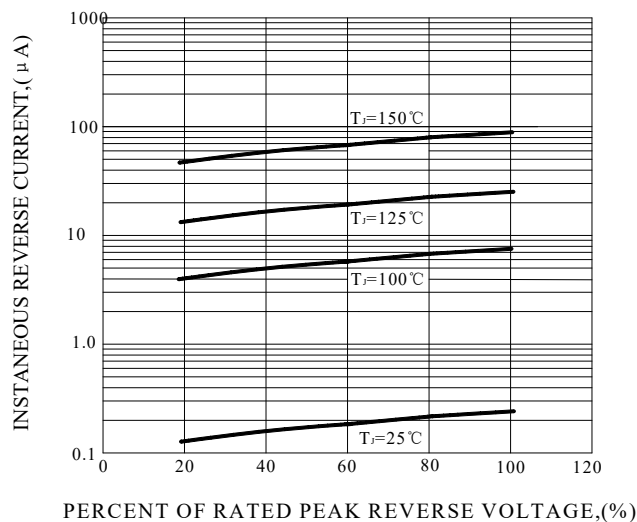
FIG.5-TYPICAL REVERSE CHARACTERISTICS
