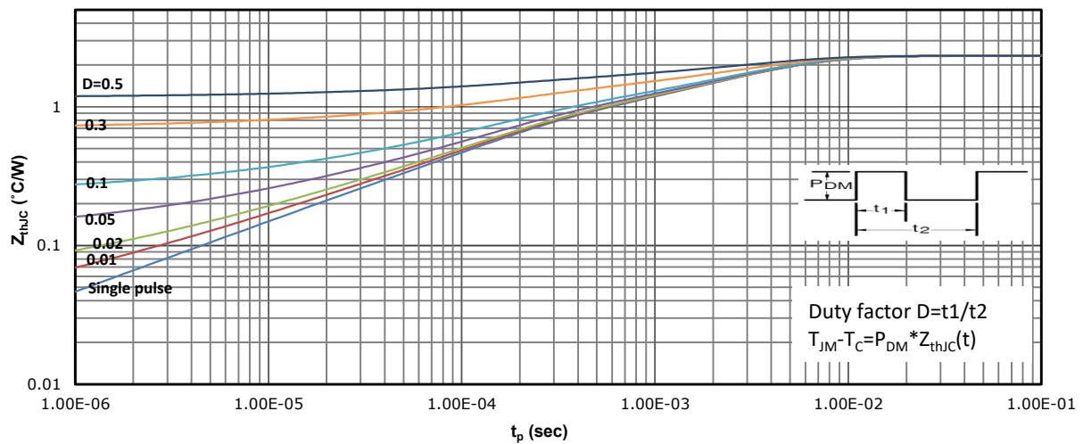
Fig 15: Max. Transient Thermal Impedance R_{JC}
