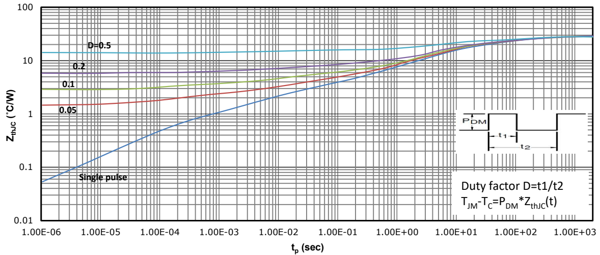
Fig 15: Max. Transient Thermal Impedance R_{JC}
