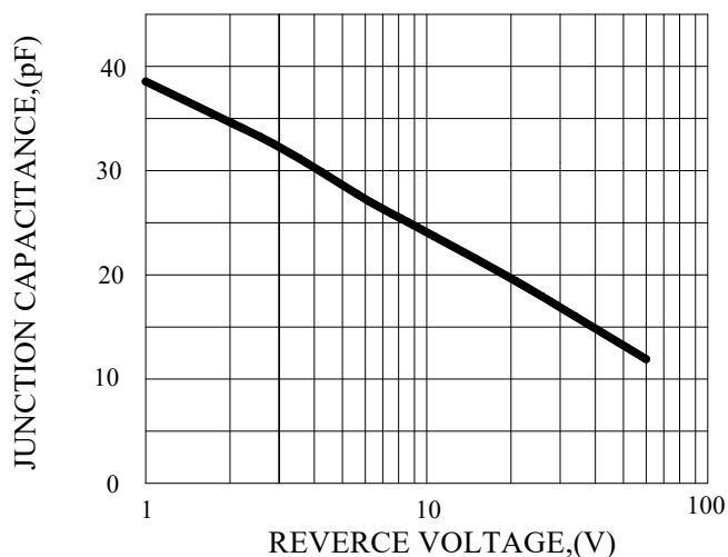
FIG.5-TYPICAL JUNCTION CAPACITANCE
