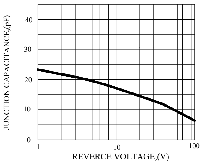
FIG.6-TYPICAL JUNCTION CAPAOTANCE
