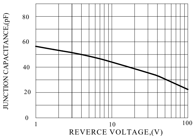
FIG.6-TYPICAL JUNCTION CAPACITANCE
