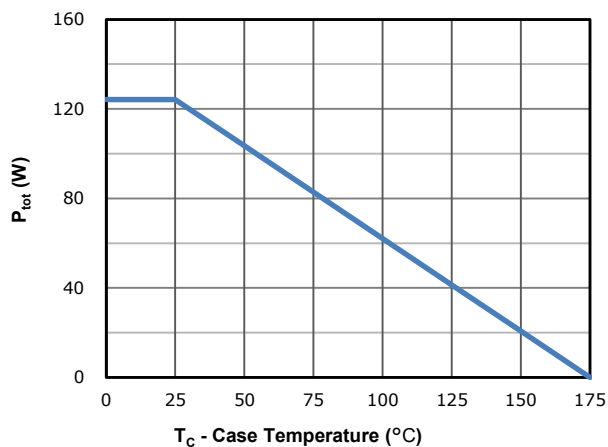
Fig 11: Power Dissipation
