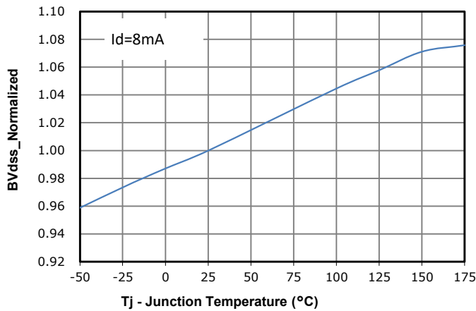
Fig 7: BVdss vs. Temperature
