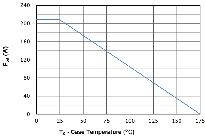
Fig 11: Power Dissipation
