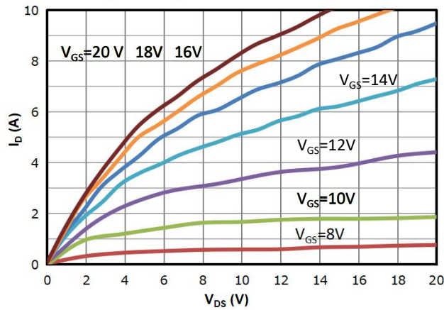
Fig 1: Output Characteristics-25°C
