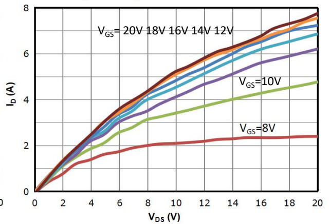
Fig 2: Output Characteristics-175°C
