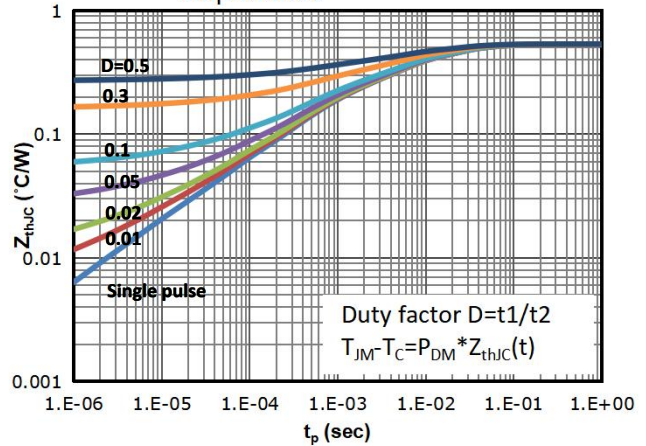
Fig 6: Max. Transient Thermal Impedance
