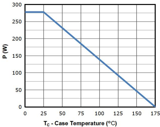
Fig 5: Power Dissipation
