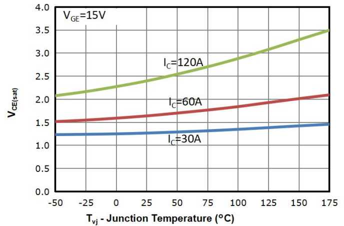
Fig 6: V_{CE(sat)} vs. Temperature
