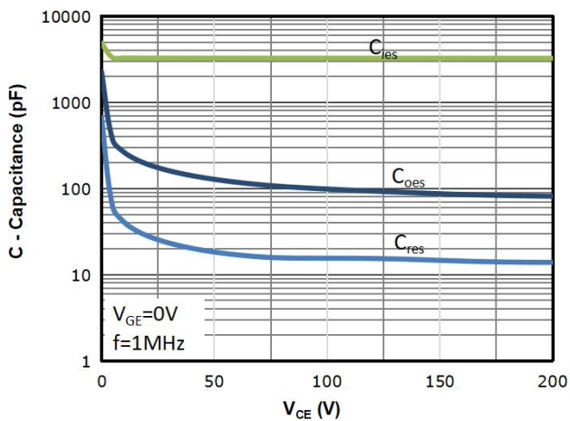
Fig 11: Capacitance Characteristics
