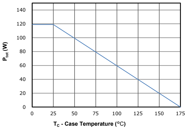
Fig 11: Power Dissipation
