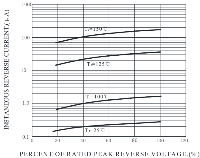
FIG.5-TYPICAL REVERSE CHARACTERISTICS
