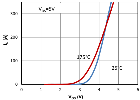
Fig 2: Transfer Characteristics
