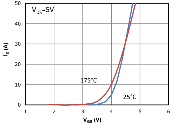
Fig 2: Transfer Characteristics
