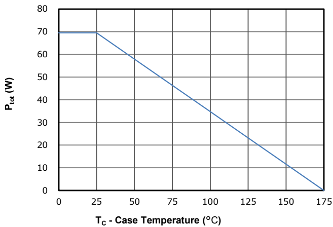
Fig 11: Power Dissipation
