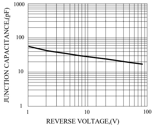
FIG.4-TYPICAL JUNCTION CAPACITANCE
