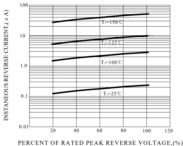
FIG.5-TYPICAL REVERSE CHARACTERISTICS
