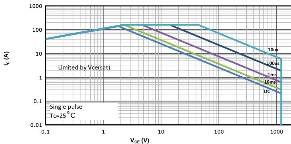
Fig 17: Safe Operating Area
