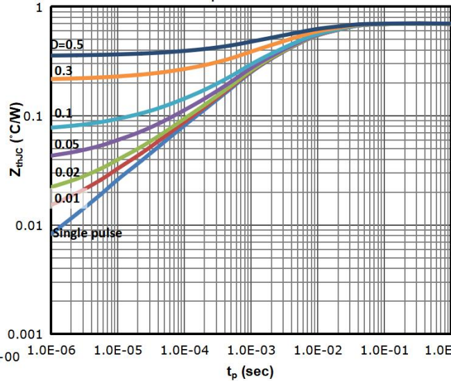
Fig 16: Diode Max. Transient Thermal Impedance
