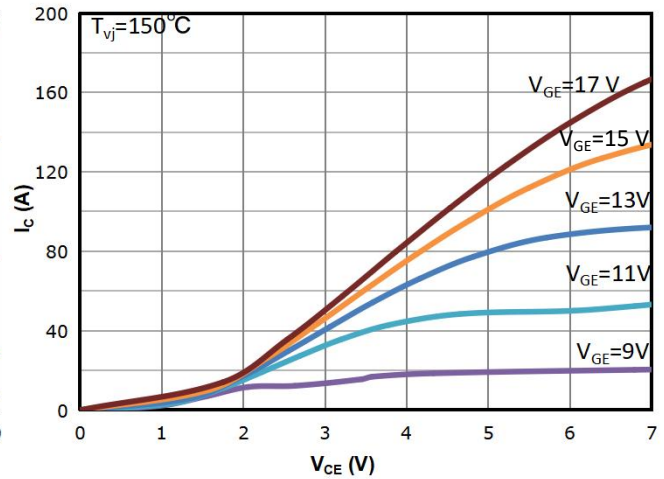
Fig 2: Output Characteristics
