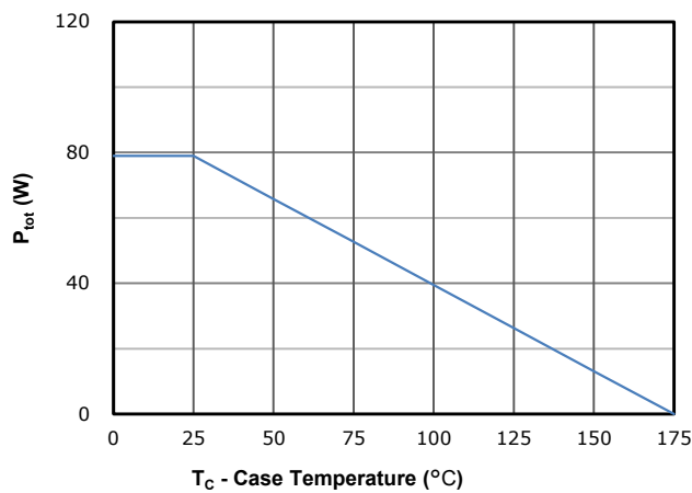
Fig 11: Power Dissipation
