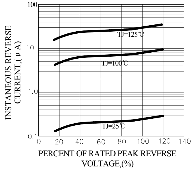
FIG.4-TYPICAL REVERSE CHARACTERISTICS
