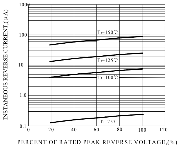
FIG.5-TYPICAL REVERSE CHARACTERISTICS
