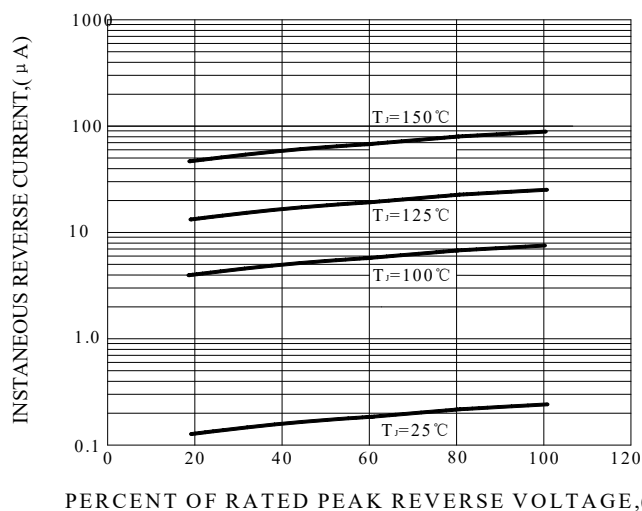
FIG.5-TYPICAL REVERSE CHARACTERISTICS
