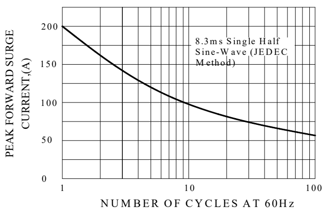
FIG.3-MAXIMUN NON-REPETITIVE FORWARD SURGE CURRENT
