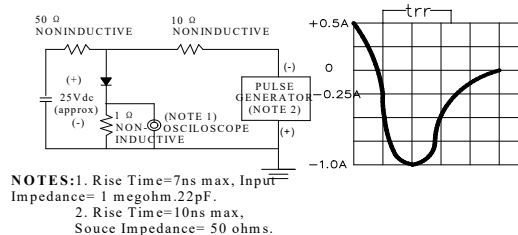
FIG.6-TEST CIRCUIT DIAGRAM AND REVERSE RECOVERY TIME CHARACTERISTIC
