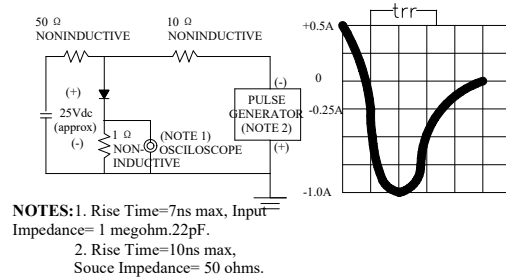
FIG.6-TEST CIRCUIT DIAGRAM AND REVERSE RECOVERY TIME CHARACTERISTIC
