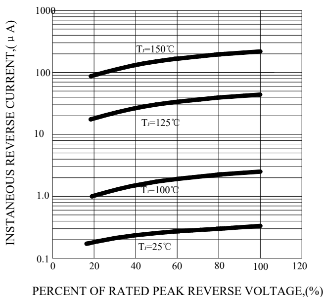
FIG.5-TYPICAL REVERSE CHARACTERISTICS
