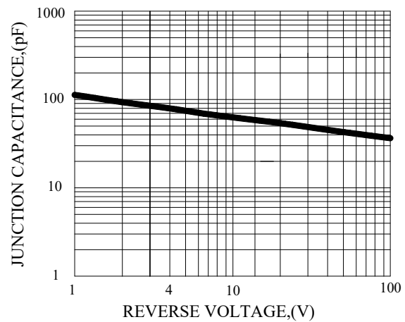
FIG.4-TYPICAL JUNCTION CAPACITANCE
