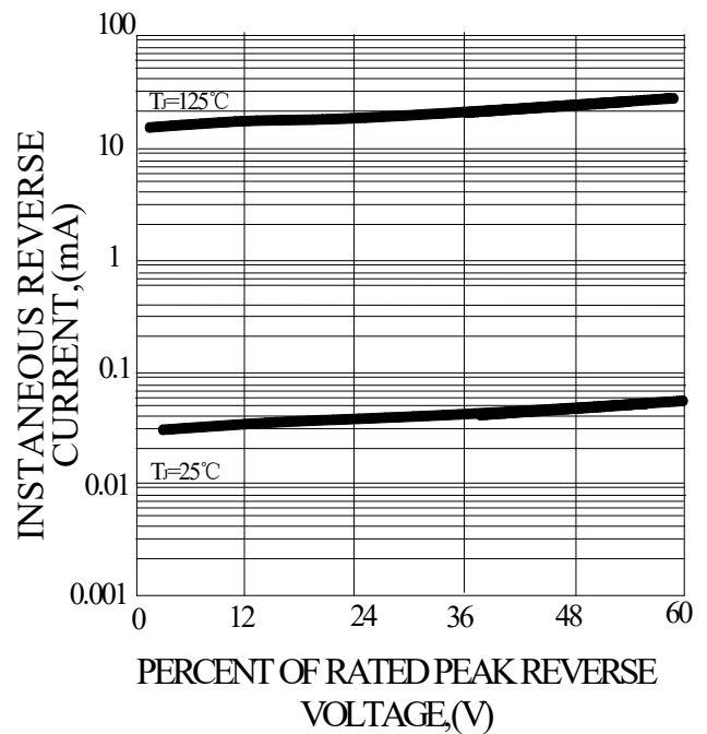
FIG.4-TYPICAL REVERSE CHARACTERISTICS
