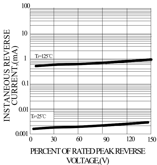
FIG.4-TYPICAL REVERSE CHARACTERISTICS
